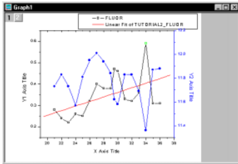
Figure 2.11: Linear Fit of Data with Mask Disabled (1 Fit Line)
